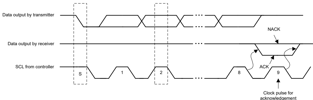
Figure 8-32. I²C Acknowledgment
