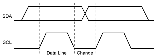
Figure 8-31. I²C Bit Transfer
