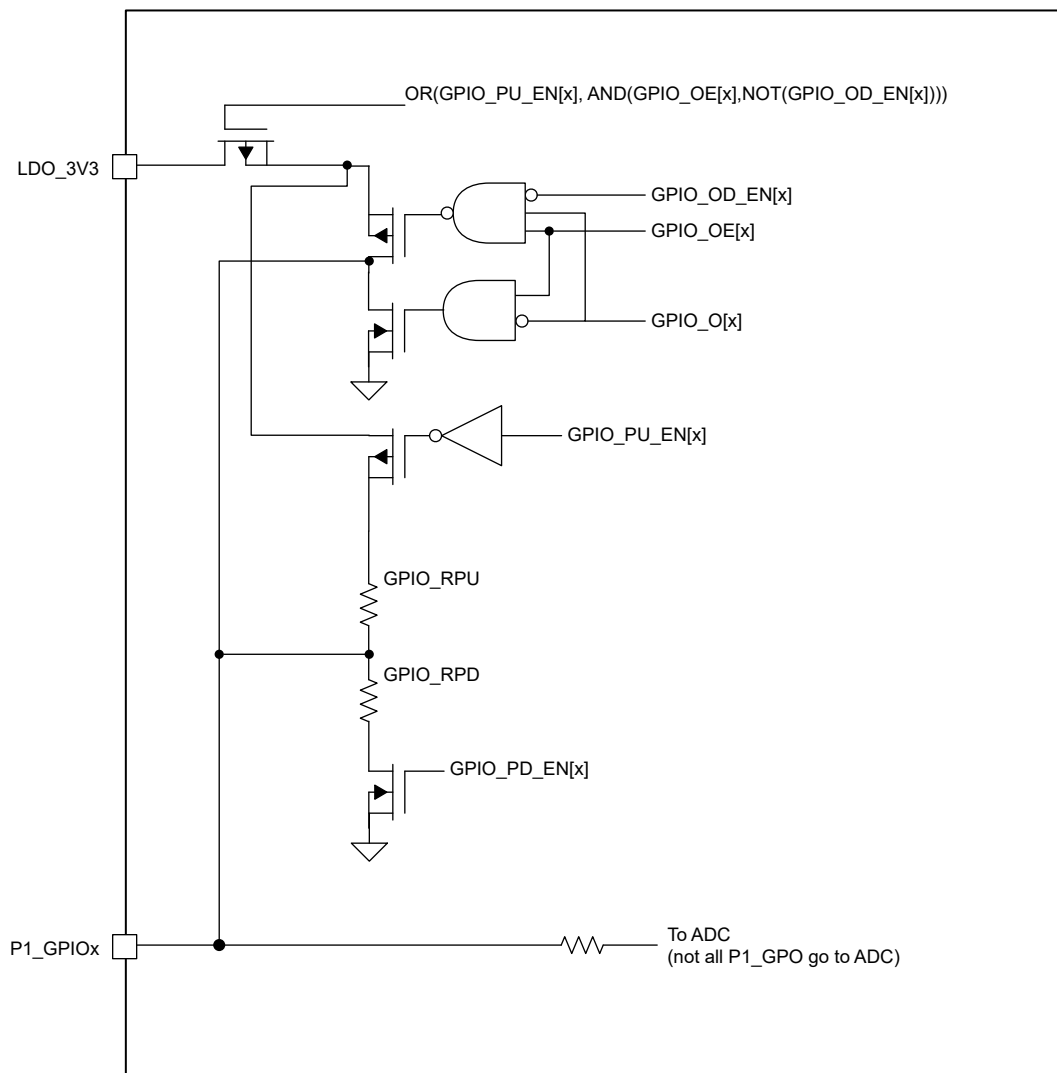
Figure 8-26. P1_GPOx Buffer
