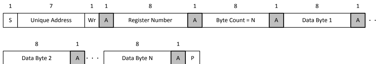
Figure 8-33. I²C Unique Address Write Register Protocol
