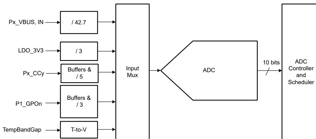
Figure 8-22. SAR ADC
