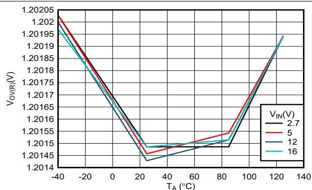
Figure 6-11. OVLO Rising Threshold vs Temperature
