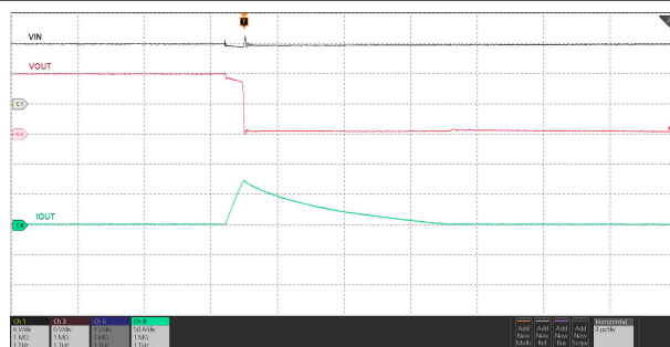
Figure 6-35. Circuit-Breaker Response
