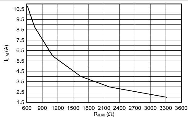
Figure 6-13. Overcurrent Threshold vs ILM Resistor
