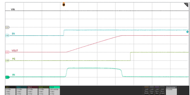
Figure 6-29. Start-Up with Supply
