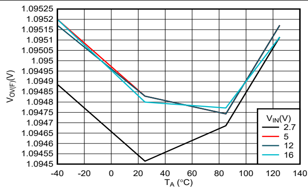
Figure 6-12. OVLO Falling Threshold vs Temperature
