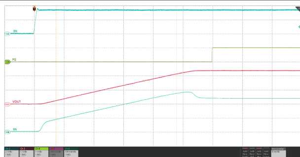
V_{IN} = 12\text{ V} , C_{OUT} = 470\text{ }\mu\text{F} , R_{OUT} = 10\text{ }\Omega , C_{dVdt} = 5100\text{ pF} , V_{EN/UVLO} stepped up to 3.3 V
