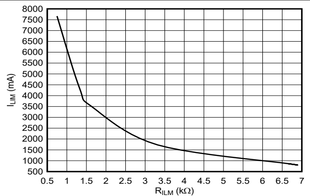
Figure 6-12. Overcurrent Threshold vs ILM Resistor
