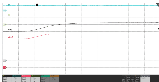
Figure 6-37. Overvoltage Clamp Response – TPS25972x
