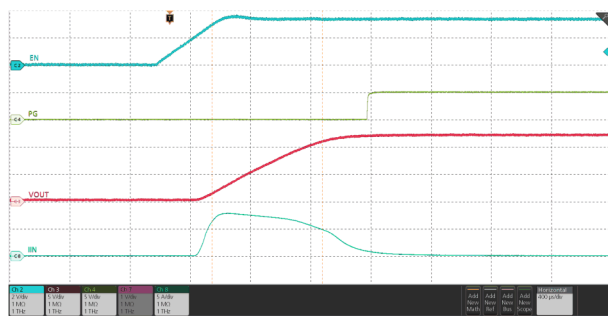
V_{IN} = 12\text{ V} , C_{OUT} = 470\text{ }\mu\text{F} , C_{dVdt} = \text{Open} , V_{EN/UVLO} stepped up to 3.3 V
