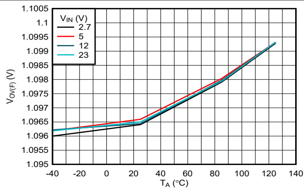
Figure 6-11. OVLO Falling Threshold vs Temperature (TPS25970x, TPS25974x Variants)
