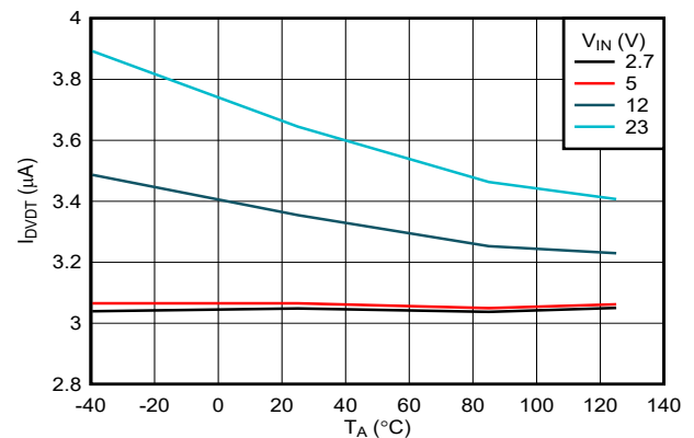
Figure 6-24. DVDT Charging Current vs Temperature
