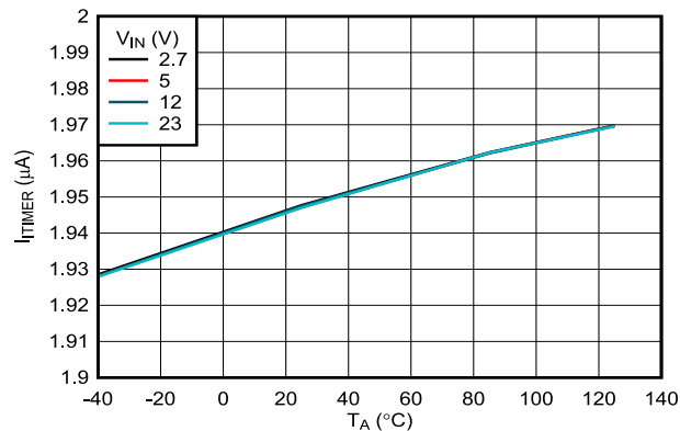
Figure 6-21. ITIMER Discharge Current vs Temperature
