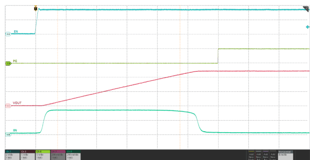
V_{IN} = 12\text{ V} , C_{OUT} = 470\text{ }\mu\text{F} , C_{dVdt} = 5100\text{ pF} , V_{EN/UVLO} stepped up to 3.3 V
