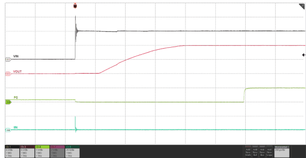
C_{OUT} = 22\text{ }\mu\text{F} , C_{dVdt} = \text{Open} , EN/UVLO connected to IN through resistor ladder, 12 V hot-plugged to IN
