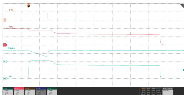
Figure 6-39. Overvoltage Clamp Response – TPS25972x
