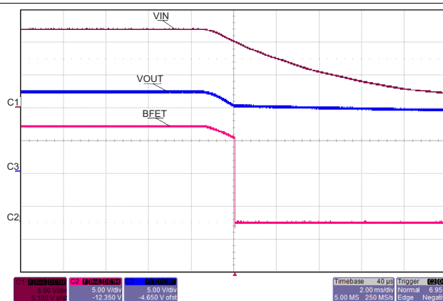
Figure 10. Transient: Turn Off Delay
