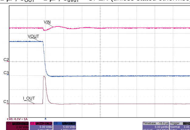
Figure 20. Short Circuit (Zoom): Fast-trip Comparator
