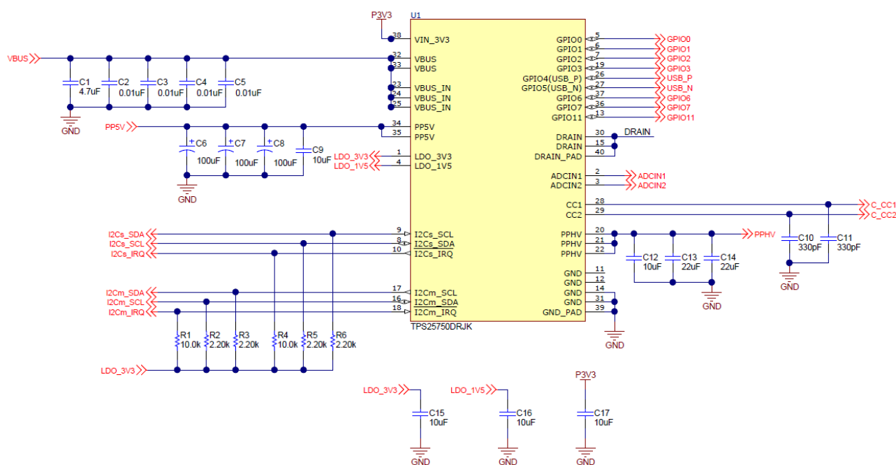
Figure 12-1. Example Schematic
