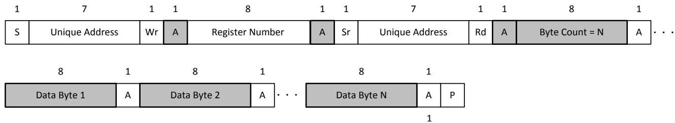
Figure 9-30. I²C Unique Address Read Register Protocol
