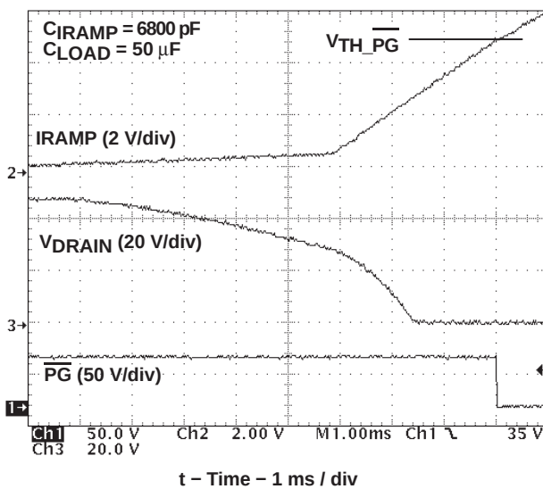
Figure 12. \overline{PG} Output Timing, Current Qualified
