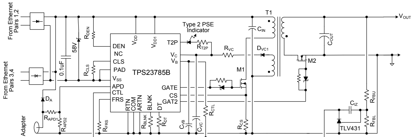
Typical Application Diagram
