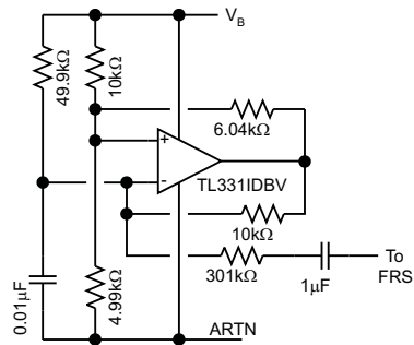
Figure 36. Frequency Dithering
