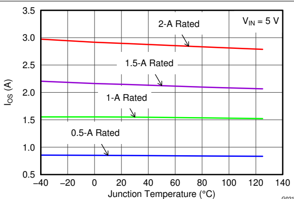
Figure 6-9. Short Circuit Current ( I_{OS} ) vs Temperature
