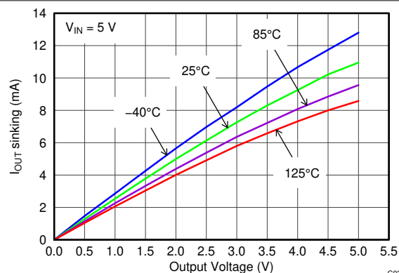
Figure 6-8. Output Discharge Current vs Output Voltage
