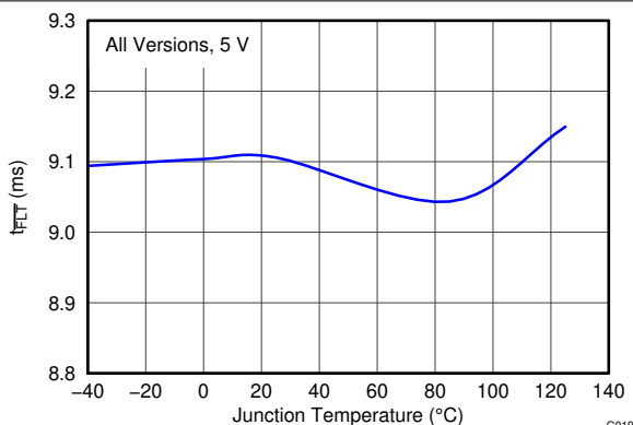
Figure 6-7. Deglitch Period ( T_{FLT} ) vs Temperature
