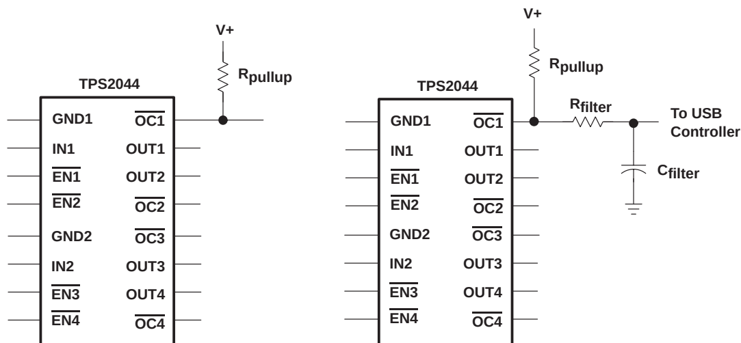
Figure 30. Typical Circuit for \overline{\text{OC}} Pin and RC Filter for Damping Inrush \overline{\text{OC}} Responses
