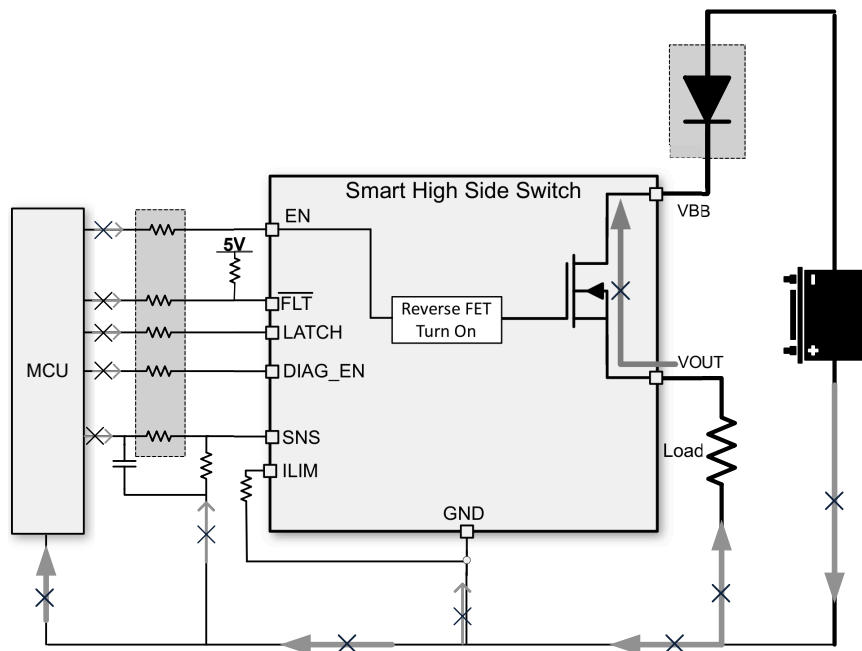
Figure 7-20. Reverse Protection With Block Diode
