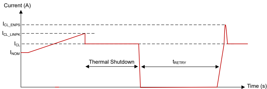
Figure 7-12. Overload Behavior (Current Creep)
