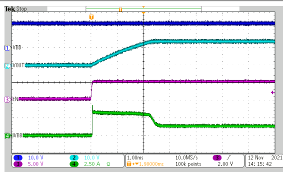
Figure 8-5. Charging a 470- \mu F Capacitor
