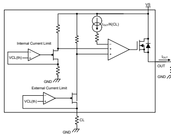
Figure 6-1. Current Limit
