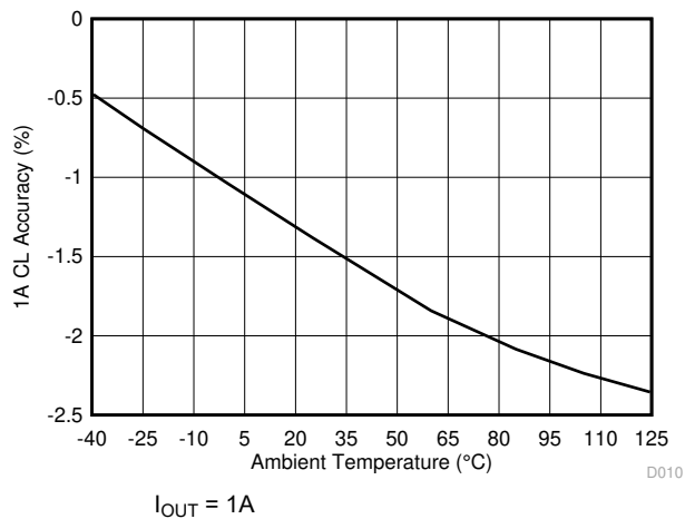
Figure 5-12. Current-Limit Accuracy at 1A
