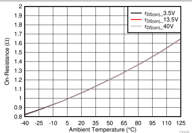
Figure 5-8. FET On-Resistance
