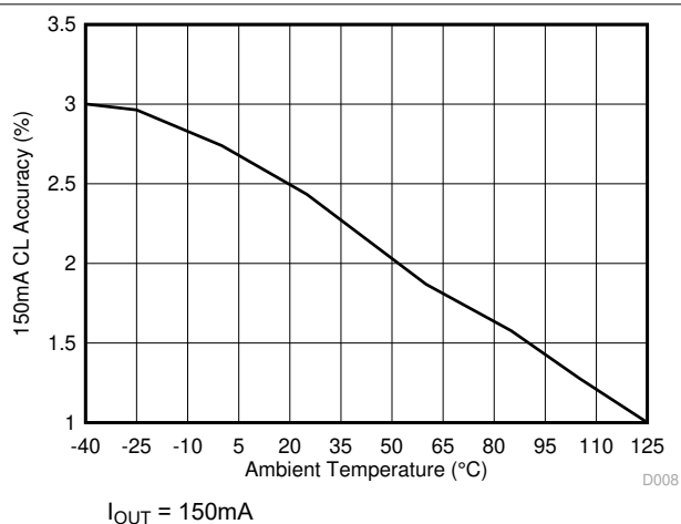
Figure 5-10. Current-Limit Accuracy at 150mA
