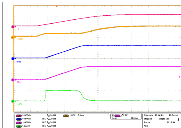
Figure 9-19. Inrush Current Profile With 1000µF at the Output ( \overline{LPM} = Low)
