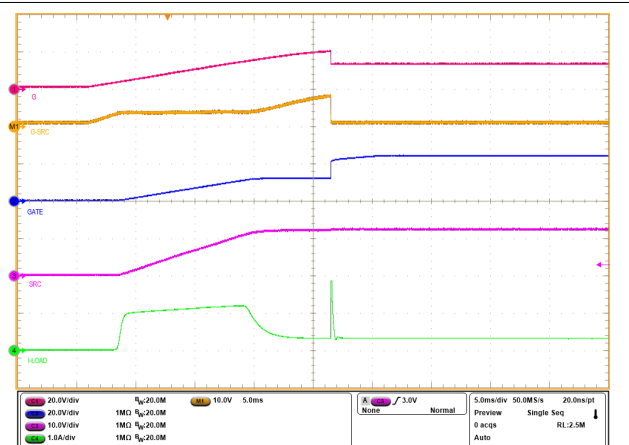
Figure 9-20. Inrush Current Profile With 1000µF at the Output and 0.5A Load ( \overline{LPM} = Low)
