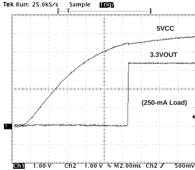
Figure 1. 5VCC Cold Start
