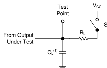
Figure 7-2. Load Circuit for Open-Drain Outputs
