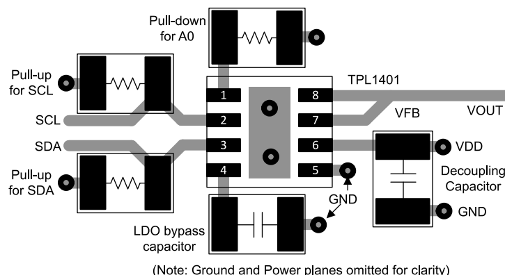
Figure 10-1. Layout Example
