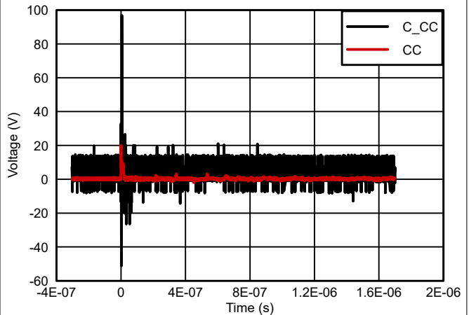
Figure 5-4. CC IEC 61000-4-2 8kV Response Waveform
