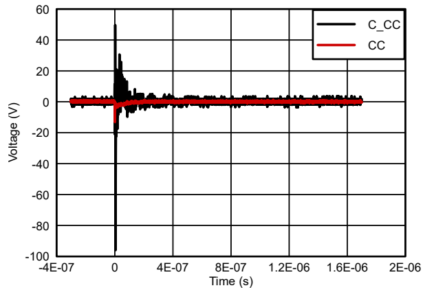
Figure 5-5. CC IEC 61000-4-2 -8kV Response Waveform
