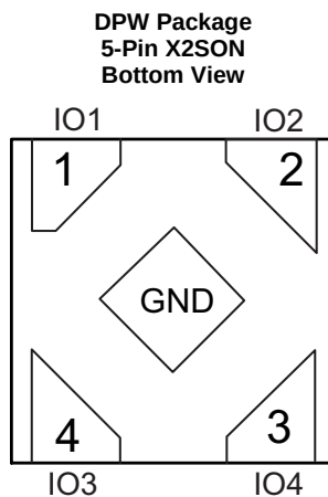
Pin Functions
