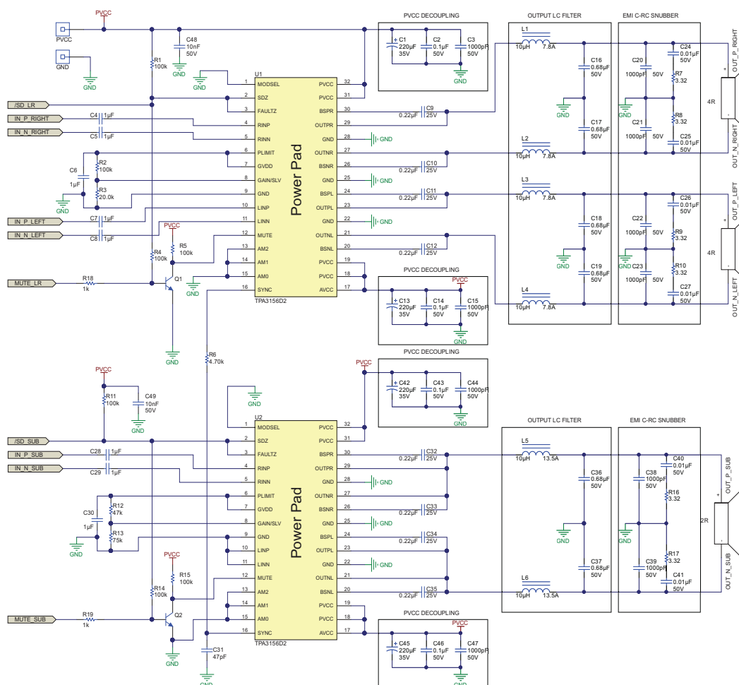
Figure 34. TPA3156D2 Schematic
