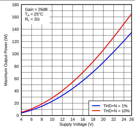
Figure 22. Maximum Output Power (PBTL) vs Supply Voltage
