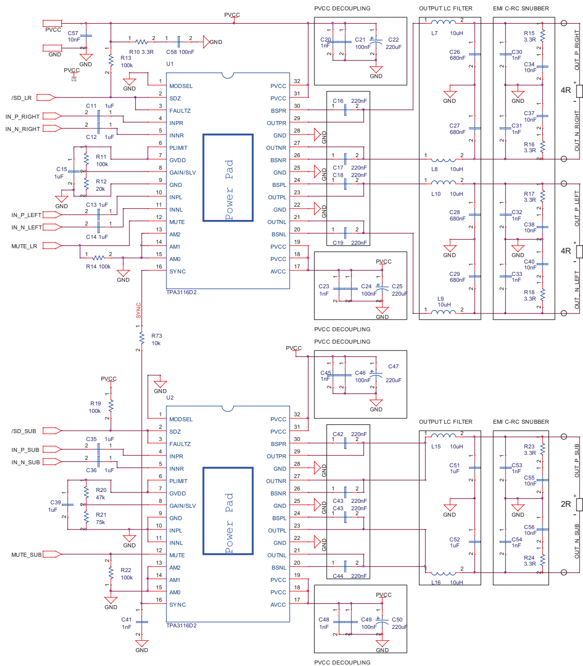
Figure 37. Schematic
