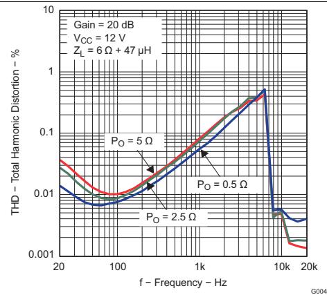
Figure 2. Total Harmonic Distortion vs Frequency (BTL)
