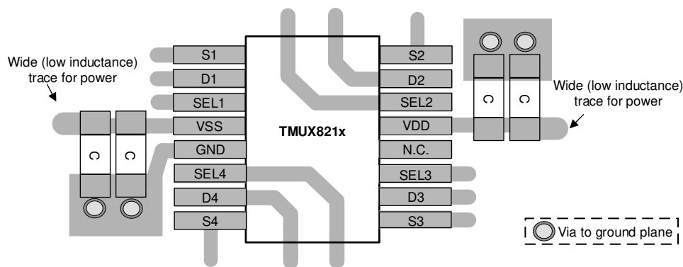
Figure 12-1. TMUX821x TSSOP Layout Example
