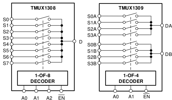
TMUX1308 and TMUX1309 Block Diagram
