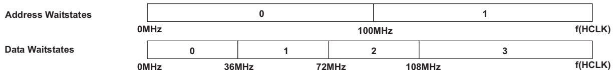
Figure 7-3. Wait States
