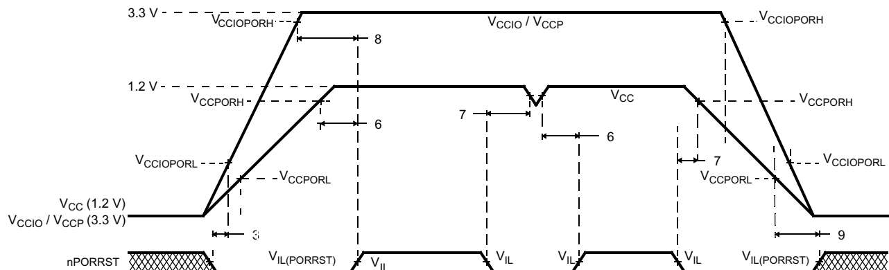
Figure 5-1. nPORRST Timing Diagram (A)
