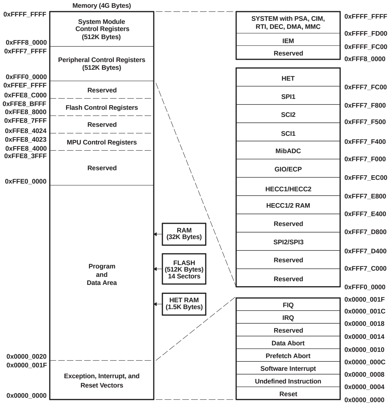
Figure 1. Memory Map
