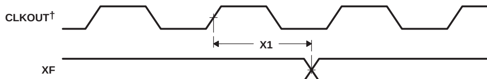
Figure 5–20. XF Timings
