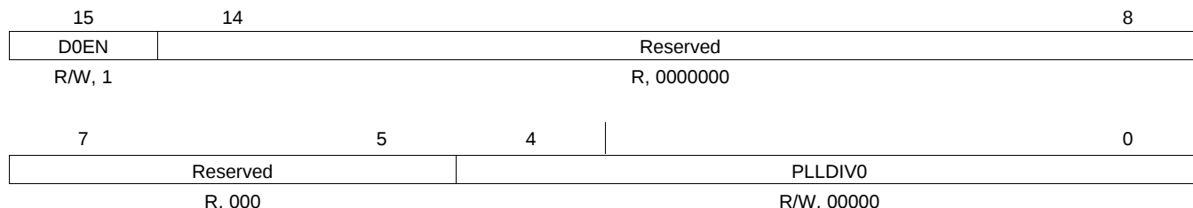
Figure 3-17. PLL Divider 0 Register Layout (0x1C8A)
