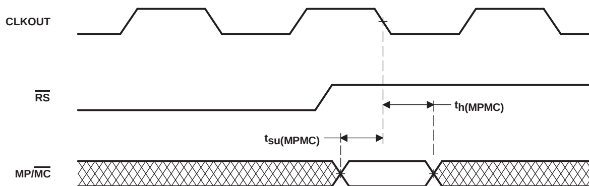
Figure 5-16. \overline{\text{MP/MC}} Timing
