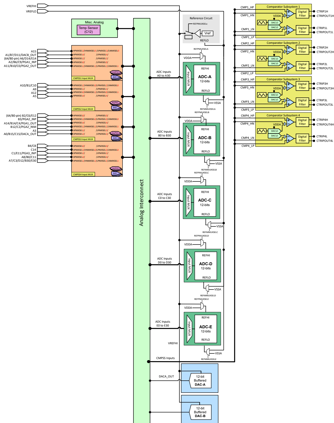
Figure 6-34. Analog Subsystem Block Diagram (80-/64-/56-Pin Packages)
