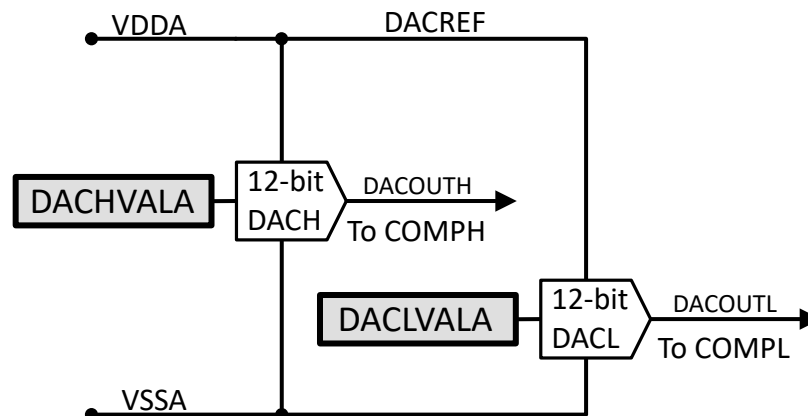
Figure 6-50. Reference DAC Block Diagram
