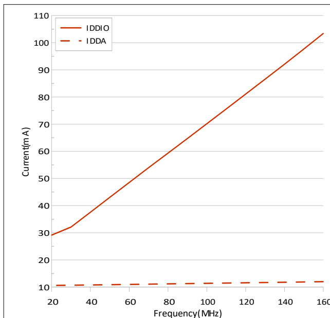
Figure 6-1. Operating Current Versus Frequency VREG Enabled
