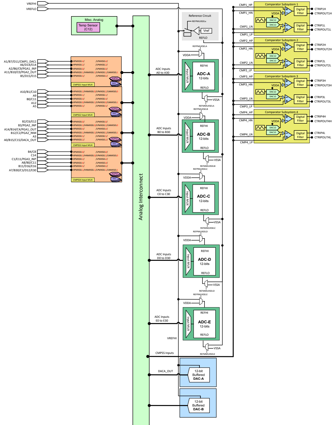
Figure 6-35. Analog Subsystem Block Diagram (100-Pin Package)
