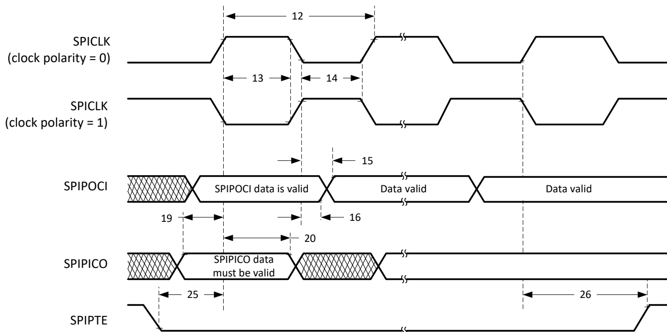
Figure 6-77. SPI Peripheral Mode External Timing (Clock Phase = 1)
