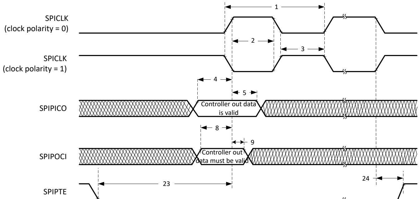
Figure 6-74. SPI Controller Mode External Timing (Clock Phase = 0)
