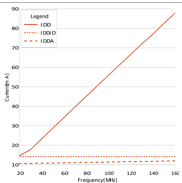
Figure 6-2. Operating Current Versus Frequency VREG Disabled
