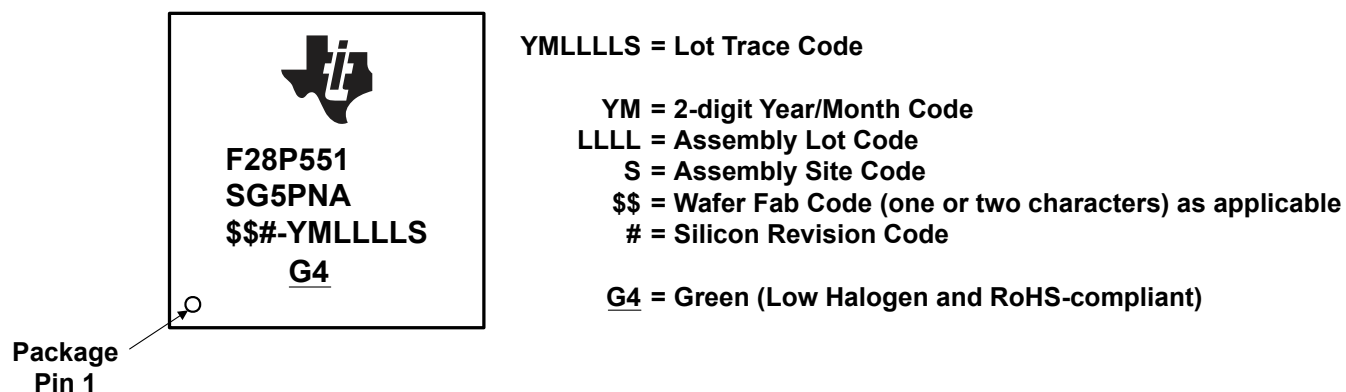
Figure 9-9. Package Symbolization for PNA Package – Non-Automotive
