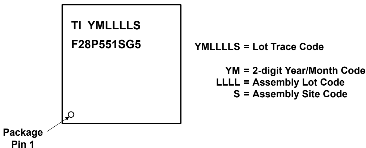
Figure 9-12. Package Symbolization for YAF Package – Non-Automotive
