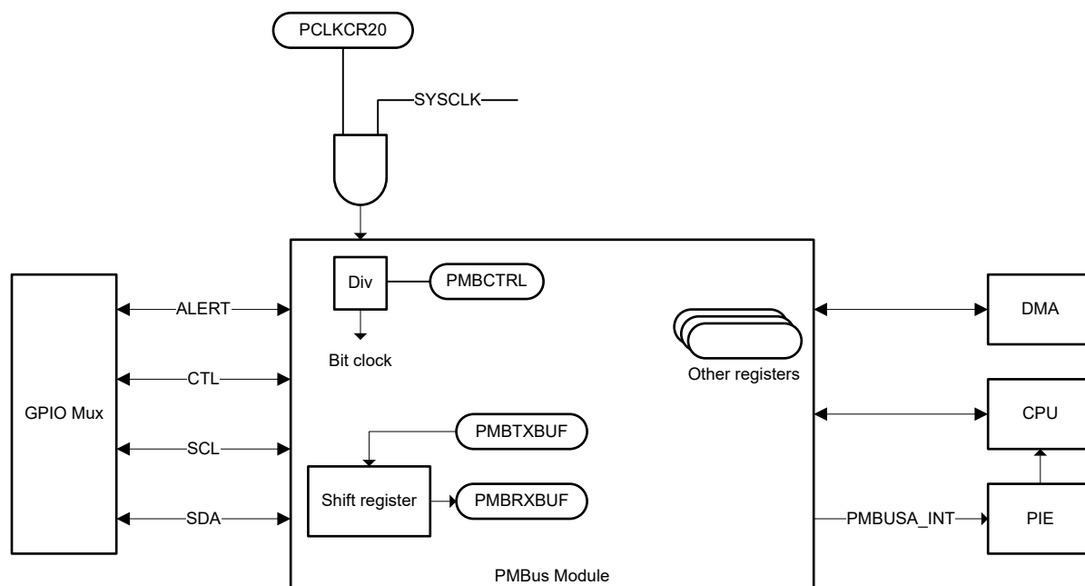
Figure 6-71. PMBus Block Diagram
