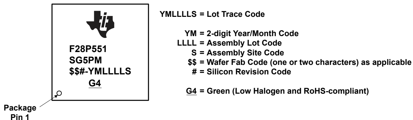
Figure 9-10. Package Symbolization for PM Package – Non-Automotive
