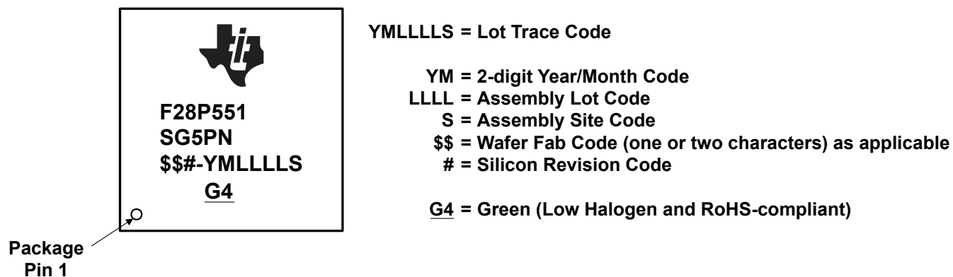
Figure 9-8. Package Symbolization for PN Package – Non-Automotive
