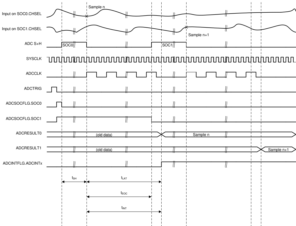
Figure 6-44. ADC Timings
