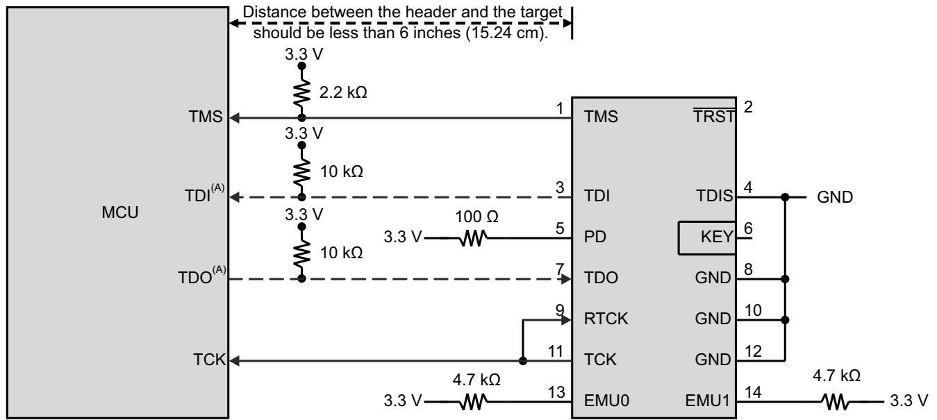
Figure 6-26. Connecting to the 14-Pin JTAG Header
