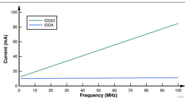
Figure 6-3. Current Versus Frequency — Internal VREG
