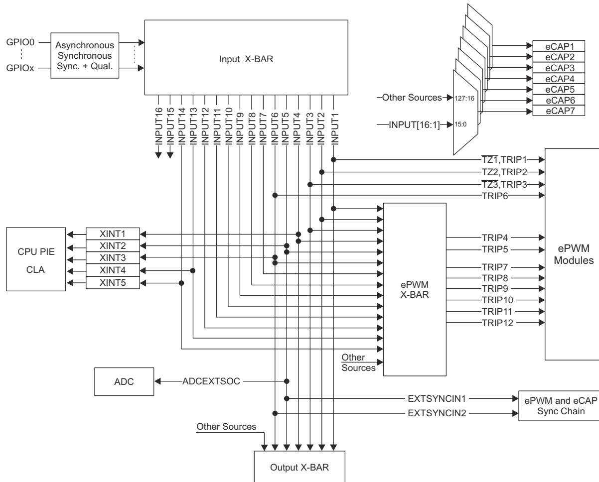
Figure 5-5. Input X-BAR
