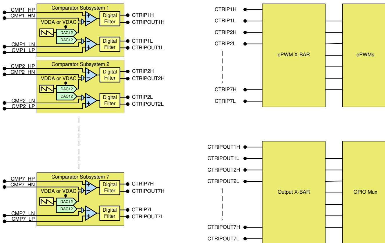
Figure 6-57. CMPSS Connectivity
