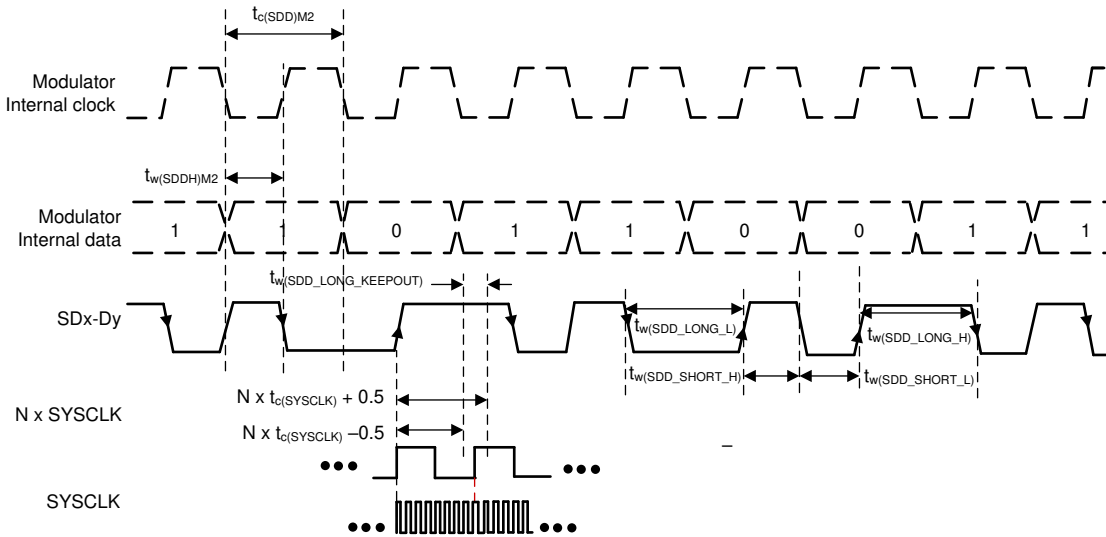
Figure 6-76. SDFM Timing Diagram – Mode 2
