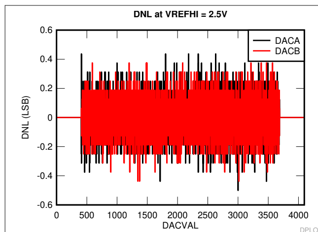
Figure 6-51. DNL
