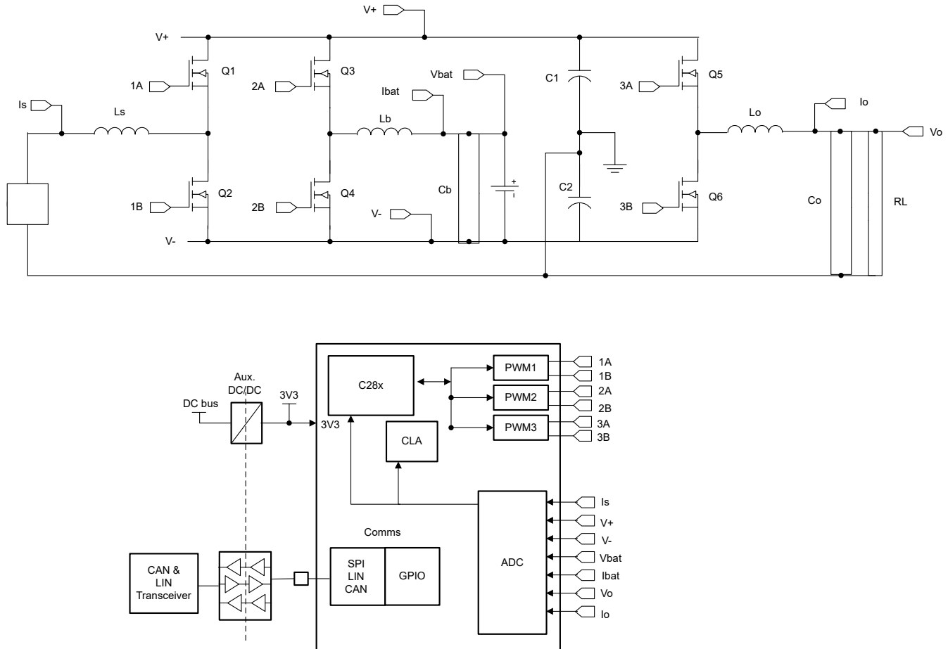
Figure 8-4. Single Phase Online UPS
