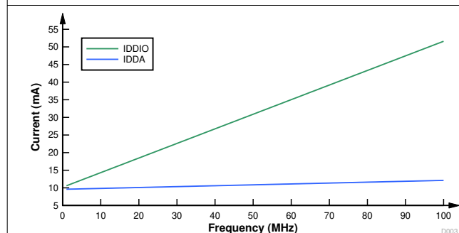
Figure 6-4. Current Versus Frequency — DCDC
