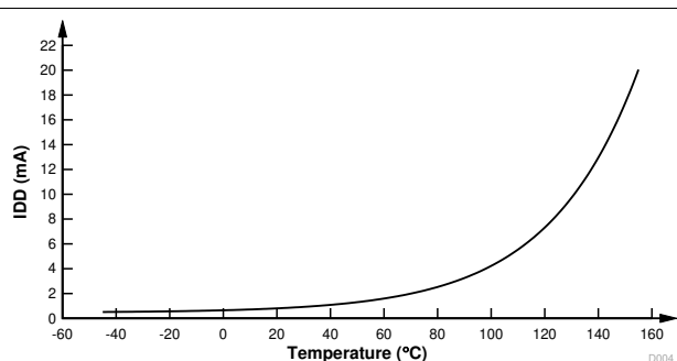
Figure 6-5. Halt Current Versus Temperature (°C)
