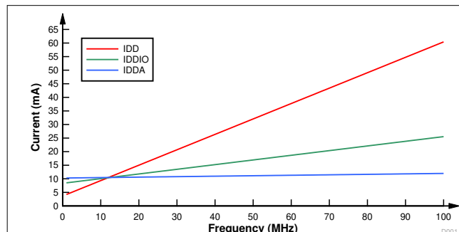
Figure 6-2. Current Versus Frequency — External Supply
