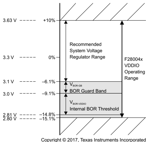
Figure 6-1. Supply Voltages
