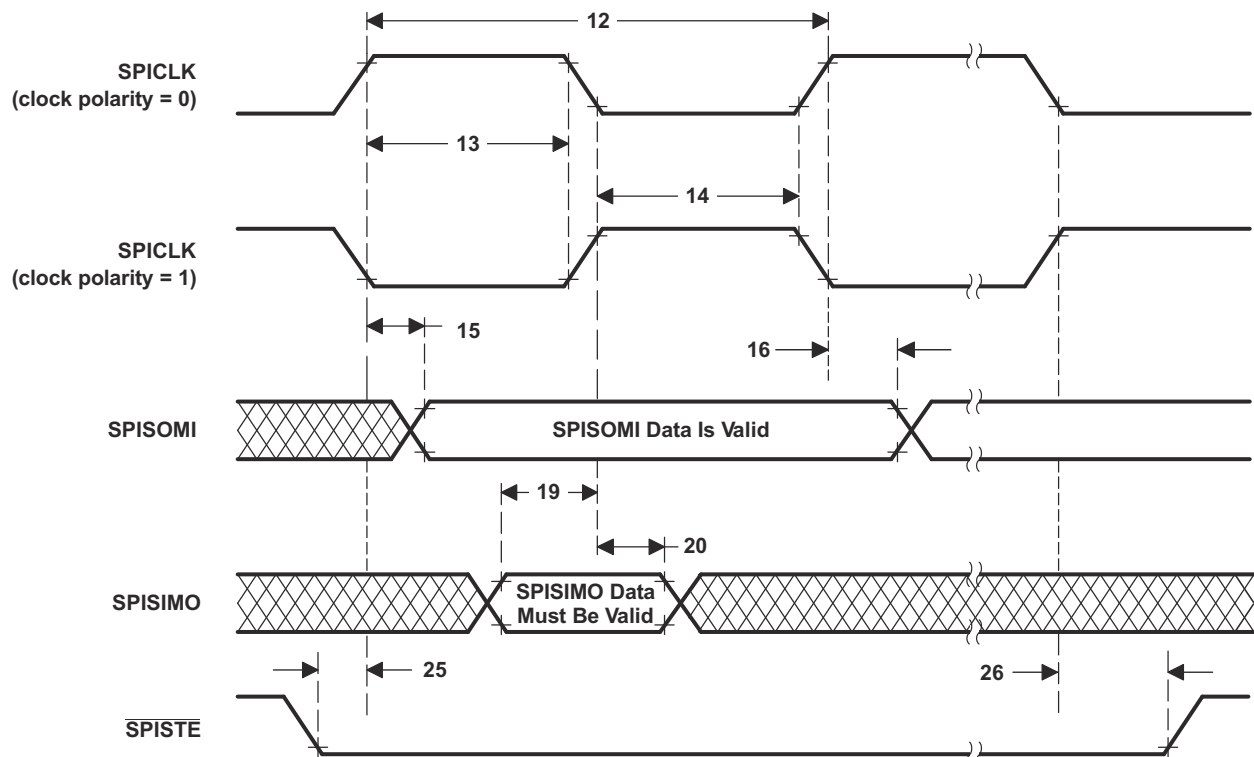
Figure 6-90. High-Speed SPI Slave Mode External Timing (Clock Phase = 0)
