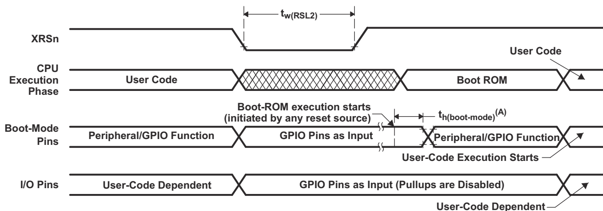
Figure 6-13. Power-on Reset
