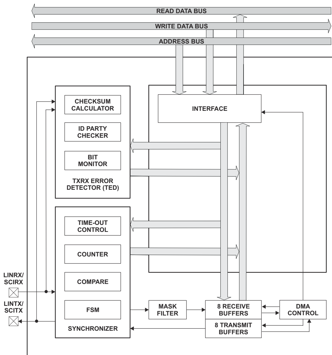
Figure 6-92. LIN Block Diagram
