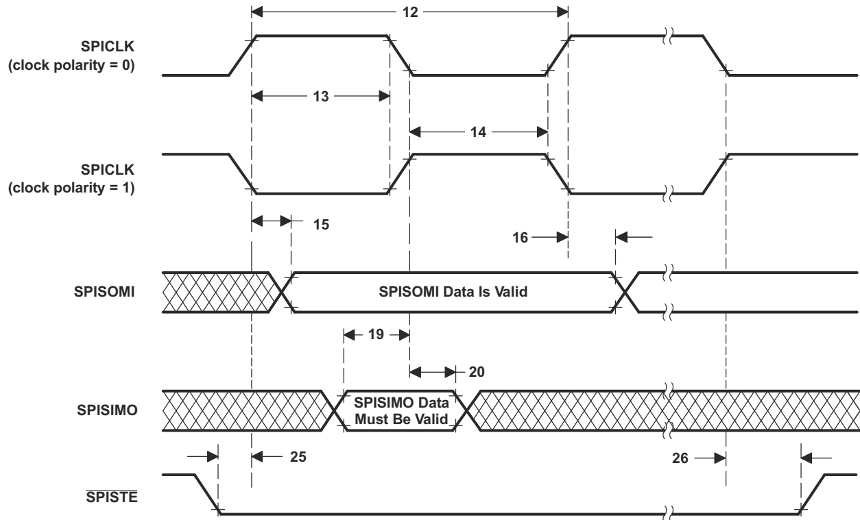
Figure 6-86. SPI Slave Mode External Timing (Clock Phase = 0)
