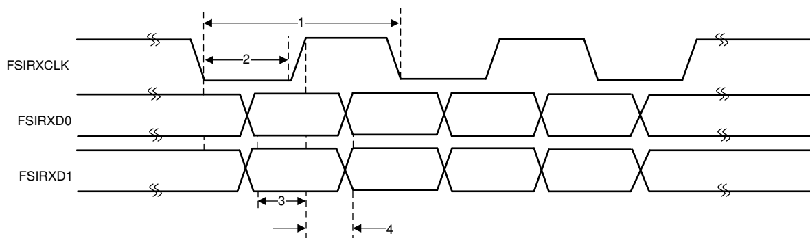
Figure 6-98. FSIRX Timings
