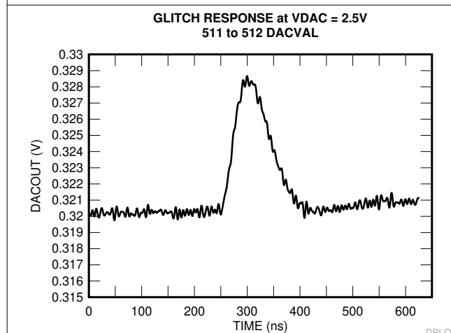
Figure 6-53. Glitch Response – 511 to 512 DACVAL
