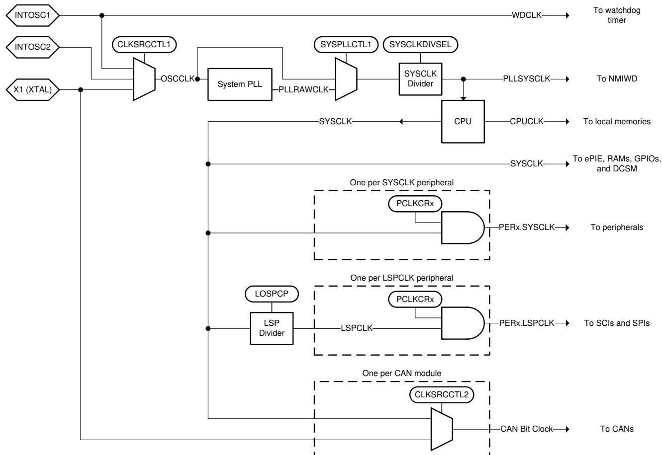
Figure 6-15. Clocking System
