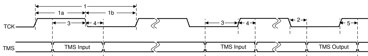
Figure 6-29. cJTAG Timing
