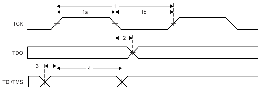
Figure 6-28. JTAG Timing
