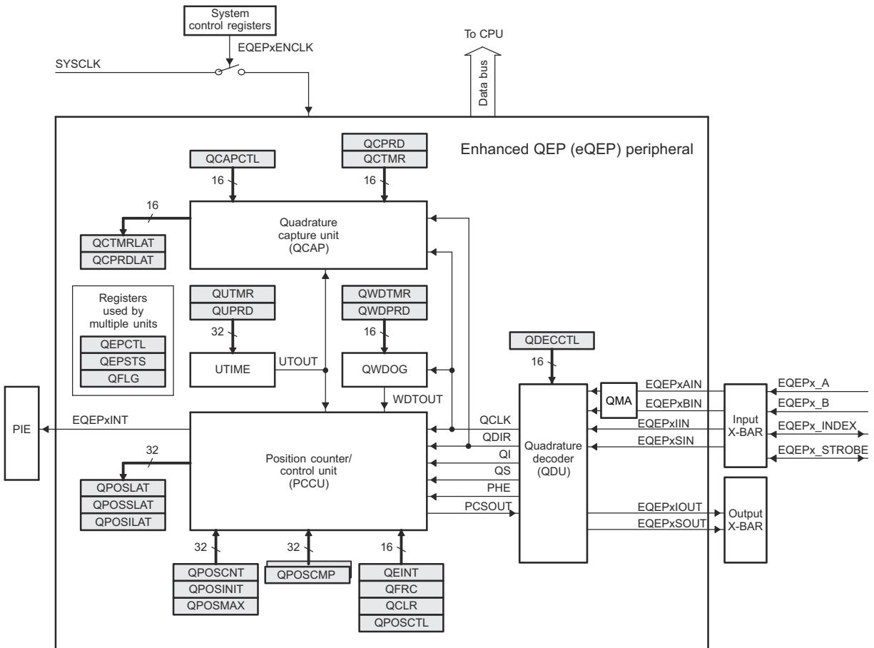
Figure 6-72. eQEP Block Diagram
