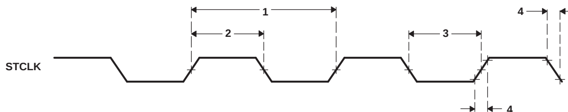
Figure 5-58. STCLK Timing
