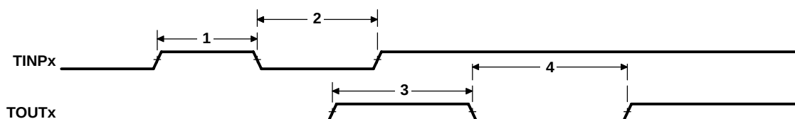
Figure 4-62. Timer Timing
