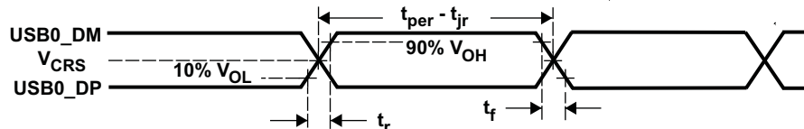
Figure 6-66. USB0 Integrated Transceiver Interface Timing
