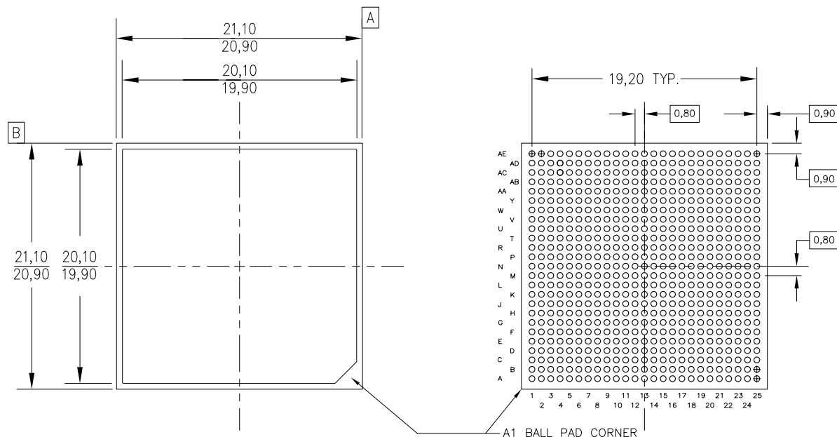
Bottom View
