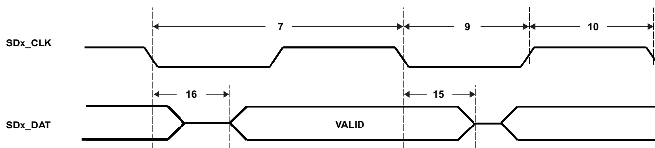
Figure 5-36. SD Data Write Timing
