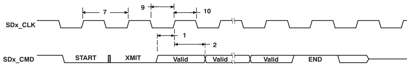
Figure 5-35. SD Host Write Timing
