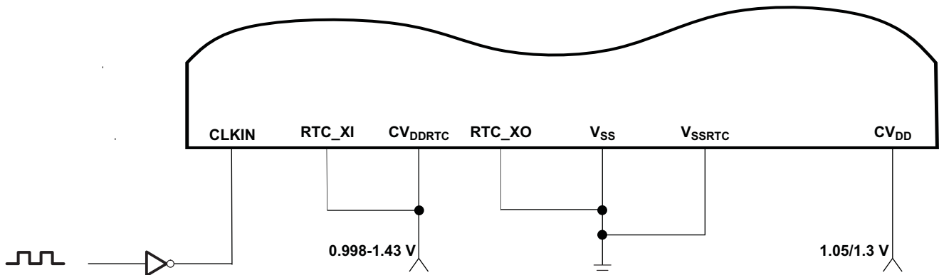
Figure 5-13. LVC MOS-Compatible Clock Input With RTC Oscillator Disabled
