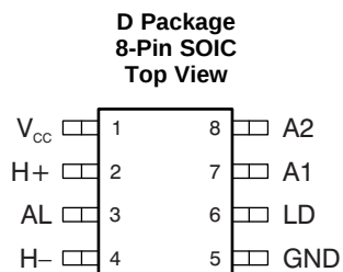
Pin Functions
