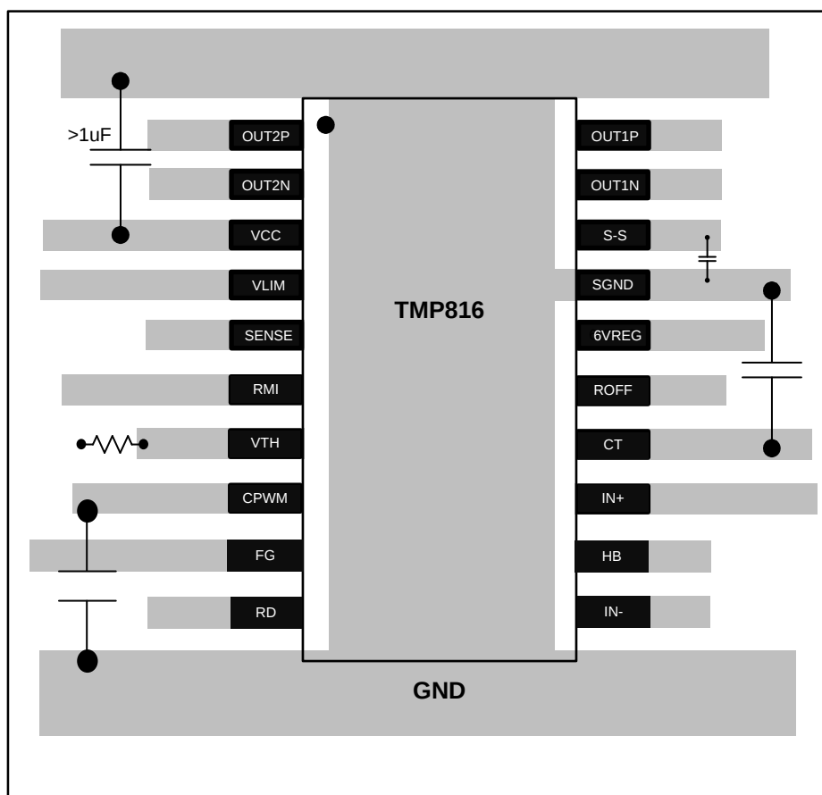
Figure 9. Recommended Layout
