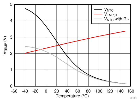
Figure 8-9. NTC With and Without a Linearization Resistor vs TMP61-Q1 Temperature Voltages
