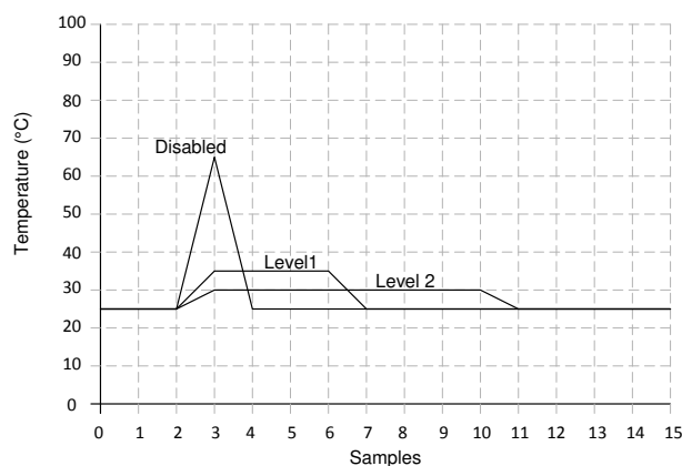
Figure 7-3. Filter Response to Impulse Inputs
