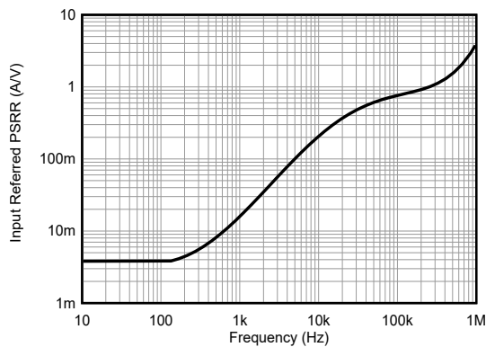
Figure 6-9. PSRR vs Frequency
