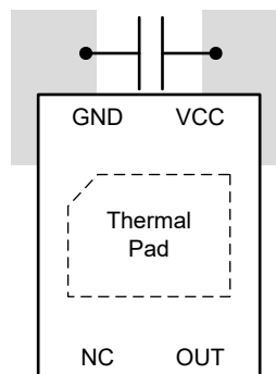
Figure 9-15. X2SON Layout Example
