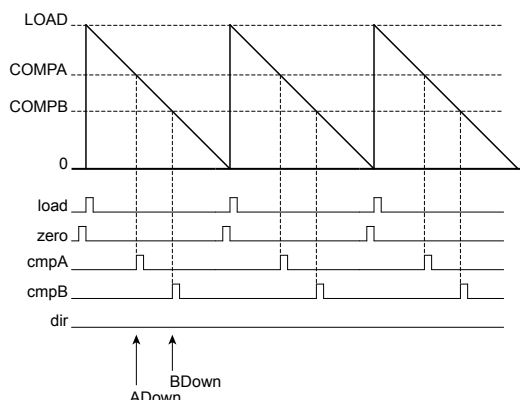
Figure 20-3. PWM Count-Down Mode
