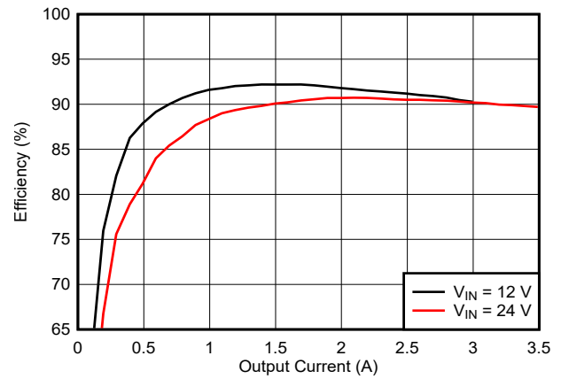
Figure 9-12. Efficiency
