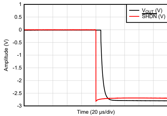
Figure 6-44. Amplifier Disable Response
