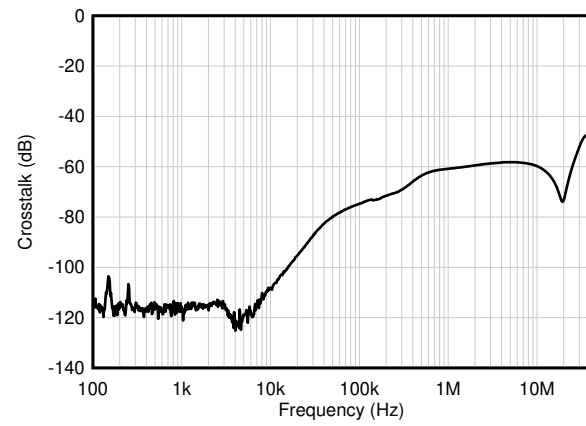
Figure 6-46. Channel Separation
