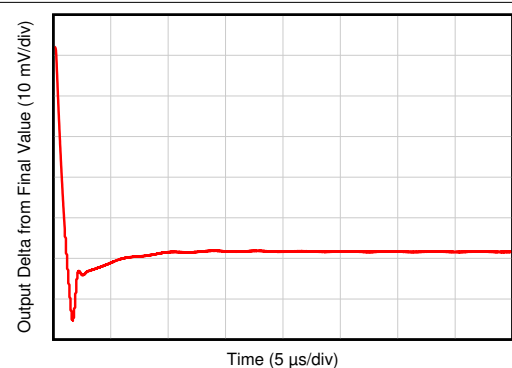
Figure 6-34. Small-Signal Step Response
