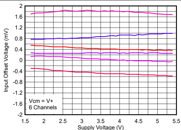
Figure 5-24. Offset Voltage vs. Supply Voltage, High VCM, 125°C
