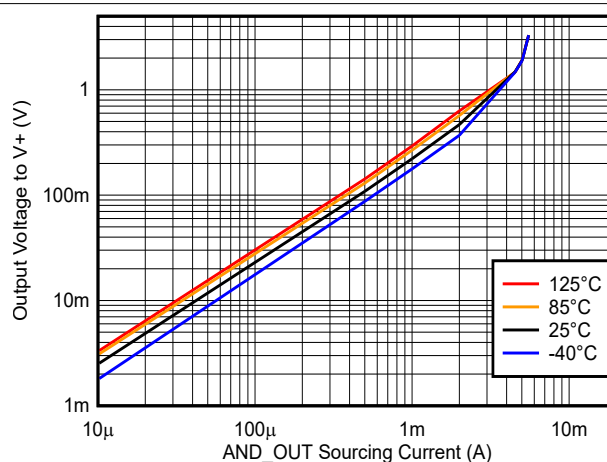
Figure 5-10. AND_OUT Sourcing Current vs. Output Voltage, 3.3V
