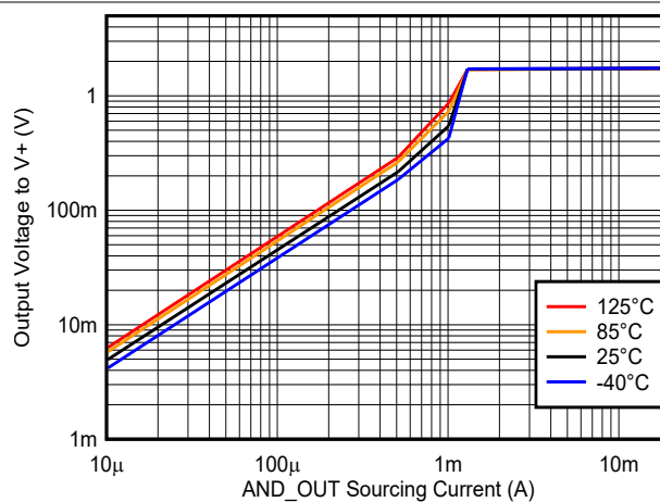
Figure 5-8. AND_OUT Sourcing Current vs. Output Voltage, 1.8V
