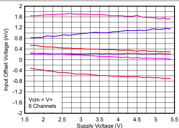
Figure 5-22. Offset Voltage vs. Supply Voltage, High VCM, 25°C
