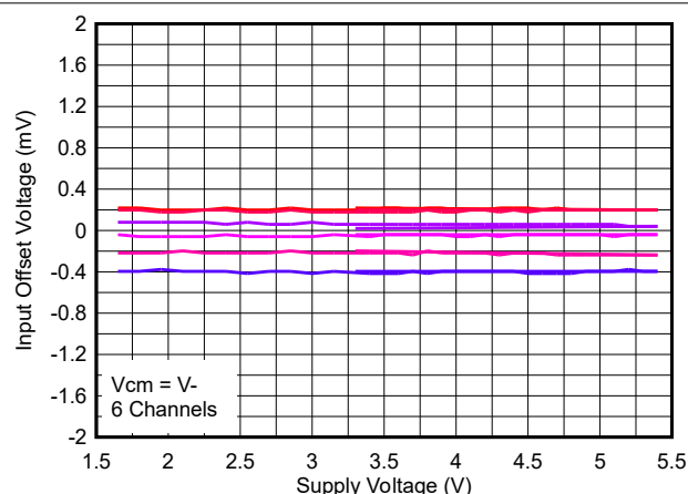
Figure 5-21. Offset Voltage vs. Supply Voltage, Low VCM, 25°C
