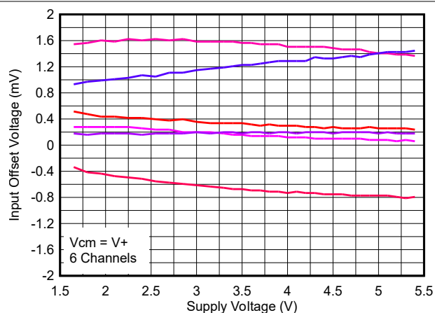
Figure 5-20. Offset Voltage vs. Supply Voltage, High VCM, -40°C
