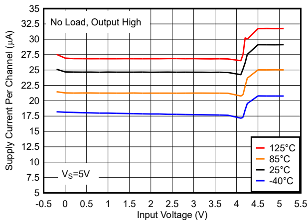
Figure 5-5. Supply Current vs. Common Mode Voltage, 5V
