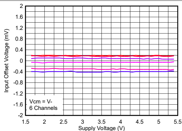
Figure 5-19. Offset Voltage vs. Supply Voltage, Low VCM, -40°C
