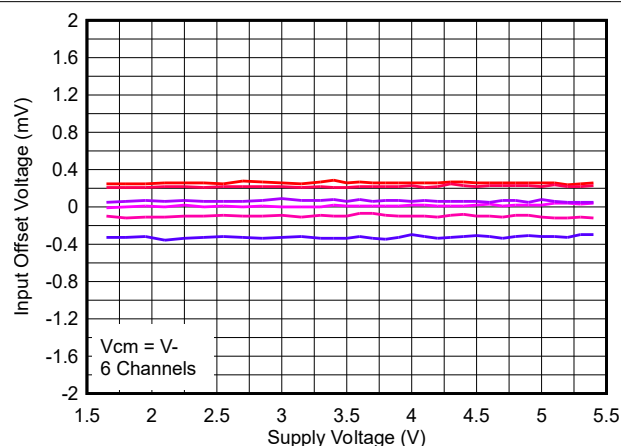
Figure 5-23. Offset Voltage vs. Supply Voltage, Low VCM, 125°C
