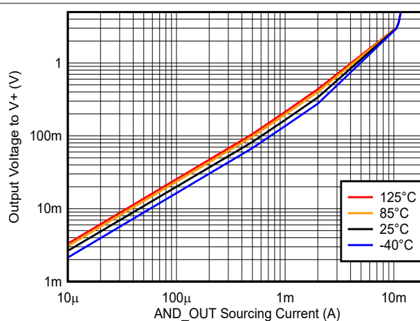
Figure 5-12. AND_OUT Sourcing Current vs. Output Voltage, 5V
