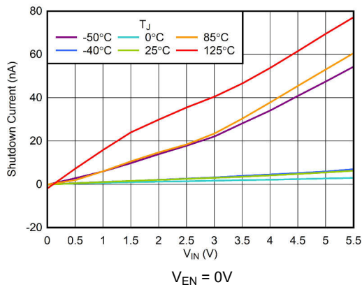
Figure 5-3. Shutdown Current vs V_{IN}
