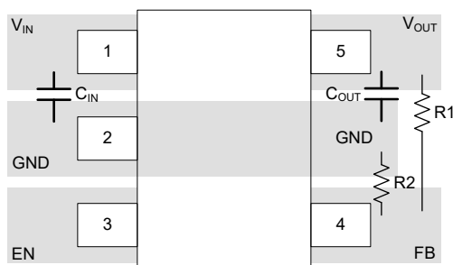
Figure 7-3. DBV Package (SOT-23) Typical Layout
