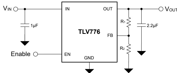
Figure 7-1. TLV776 Typical Application
