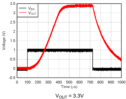
Figure 5-5. Start-Up
