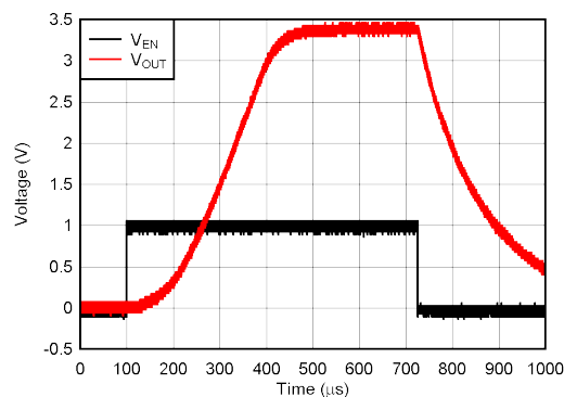
Figure 7-2. Start-Up
