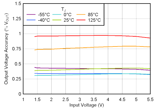
Figure 5-2. Output Voltage Accuracy vs V_{IN}
