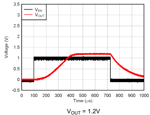
Figure 5-6. Start-Up
