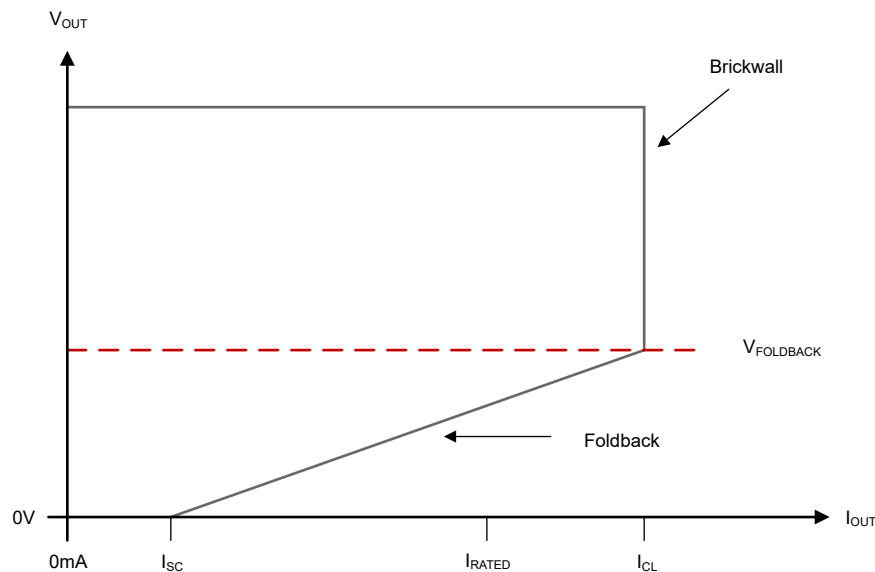
Figure 6-1. Foldback Current Limit
