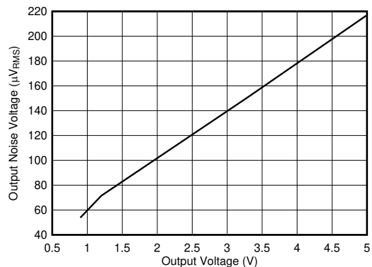
I_{OUT} = 500\text{mA} , C_{OUT} = 1\mu\text{F} , V_{RMS} \text{ BW} = 10\text{Hz to } 100\text{kHz} Figure 5-6. Output Noise Voltage vs V_{OUT}
