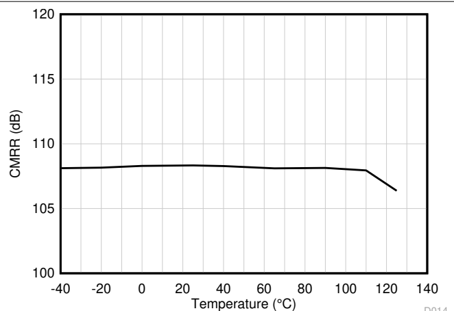
V_S = 5.5\text{ V} , V_{CM} = V_- to (V_+) - 1.2\text{ V} Figure 7-52. CMRR vs Temperature
