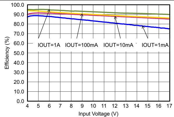
Figure 13. Efficiency With 1.25 MHz, Vout = 3.3 V
