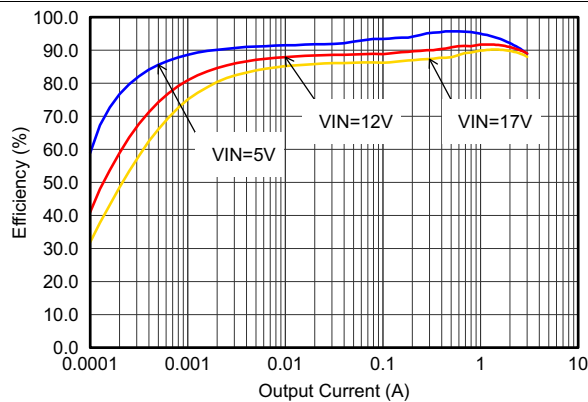
Figure 12. Efficiency With 1.25 MHz, Vout = 3.3 V
